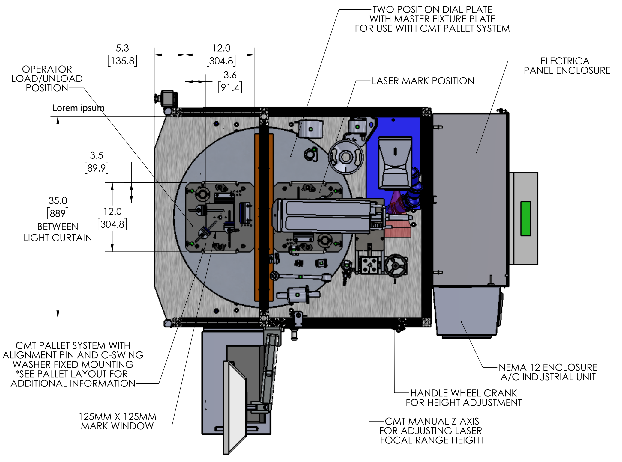
SECTION B-B TOP VIEW
