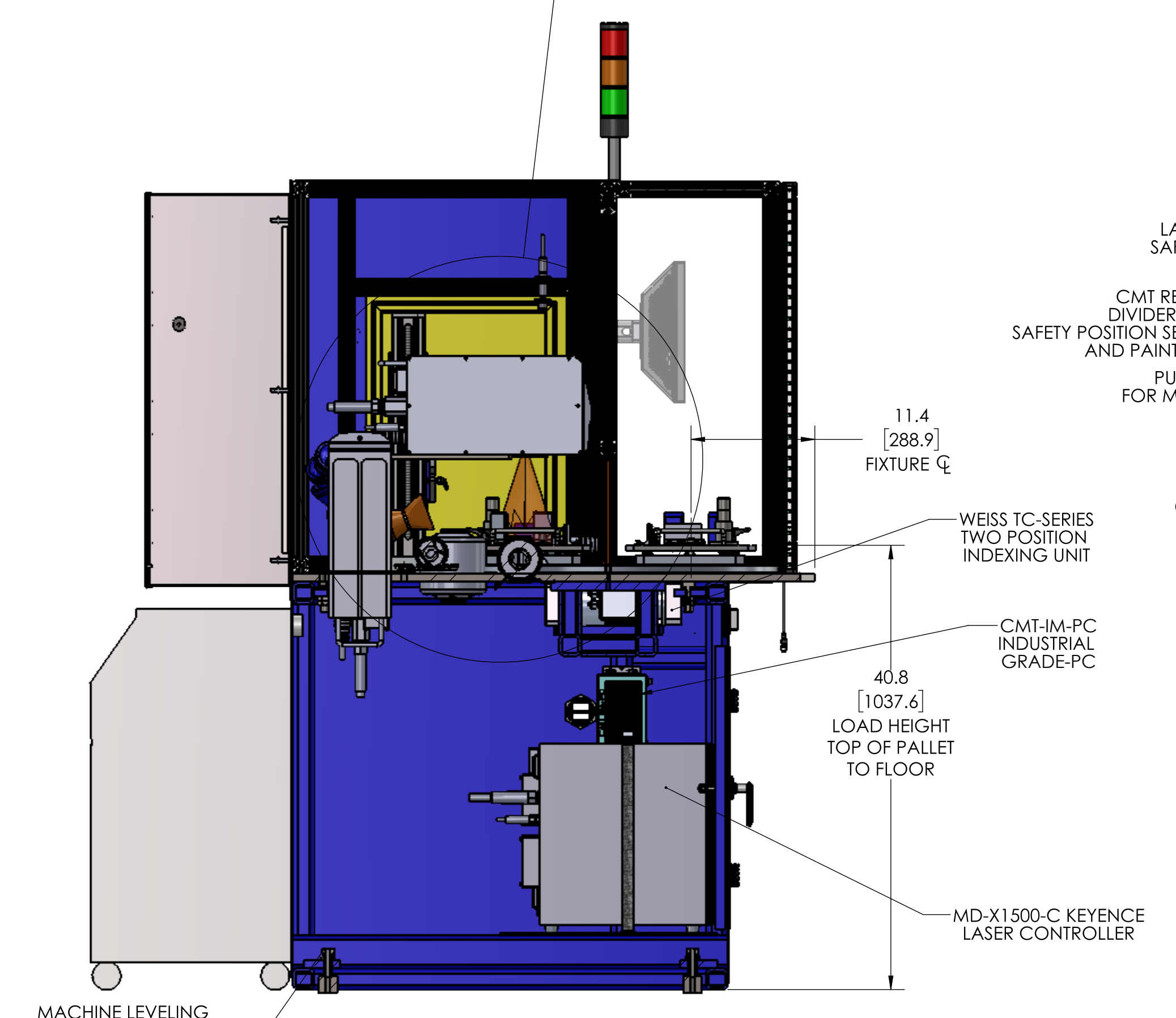
SECTION A-A LEFT SIDE VIEW
